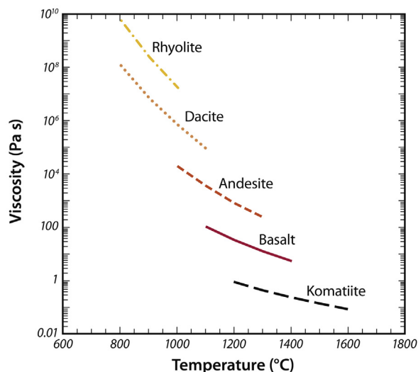
FIGURE 5.4 Viscosity as a function of temperature at 1 bar ( 10^{-4} GPa) for natural melts spanning the compositional range rhyolite to komatiite. All compositions are volatile-free. The temperature range is illustrative of typical eruption temperatures for each composition.
