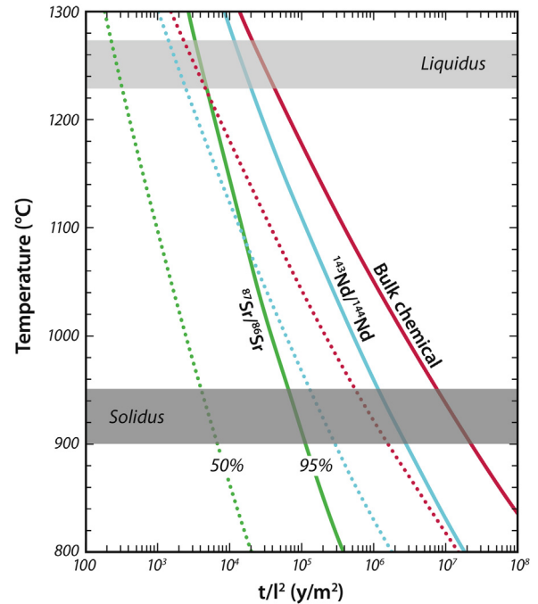
FIGURE 5.8 Effects of temperature, time, and diffusion length scale for Sr and Nd isotopic homogenization and bulk chemical homogenization of basalt with entrained blobs of rhyolite. Diffusive impedance is the time ( t ) in years over the length scale of the compositional heterogeneity ( l ) in meters squared, t/l^2 , is the diffusive impedance. Contours for 50 and 95% of the way to complete homogenization of isotopic composition and bulk chemical composition are represented by the dotted and solid curves, respectively. Approximate liquidus and solidus temperatures indicated by stippled horizontal bars delimiting the temperature interval where hybridization of basalt is likely to occur. Modified after Figure 12 in Lesher, C.E., 1994. Kinetics of Sr and Nd exchange in silicate liquids – theory, experiments, and applications to uphill diffusion, isotopic equilibration, and irreversible mixing of magmas. Journal of Geophysical Research 99, 9585–9604 with permission from John Wiley & Sons Publications.
