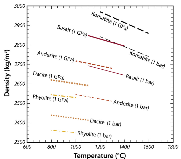
FIGURE 5.1 Melt density as a function of temperature for natural melts spanning the compositional range rhyolite to komatiite at 1 bar ( 10^{-4} GPa) and 1 GPa pressure. All compositions are volatile-free.
